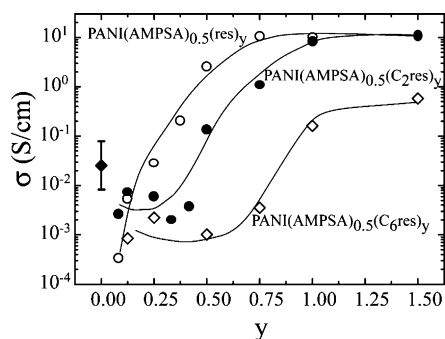
Figure 5. Room-temperature electrical conductivities for PANI(AMPSA) 0.5 (C n res) y vs y along the pressed films. The error bar indicates sample-to-sample variations. Within each sample, the error bar is smaller than the symbols.
