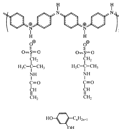
Figure 1. PANI(AMPSA) 0.5 and C_n res: resorcinol ( n = 0 ), 4-ethylresorcinol ( n = 2 ), and 4-hexylresorcinol ( n = 6 ).
